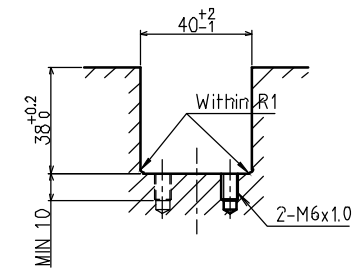
Dimension for mounting
