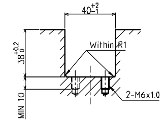
Dimension for mounting
