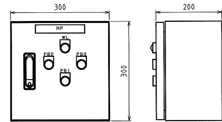
Turntable / Control panel and operation panel (Cable length: 5m)
