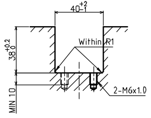
Dimension for mounting
